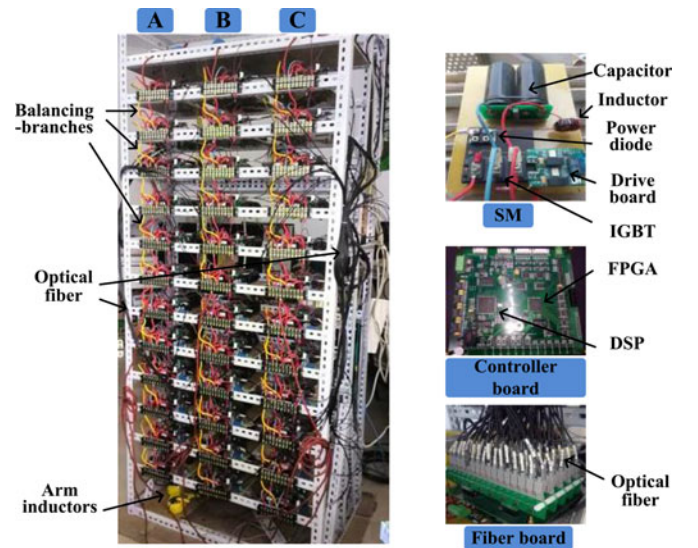
Fig. 15. Prototype of DCM 2 C.
