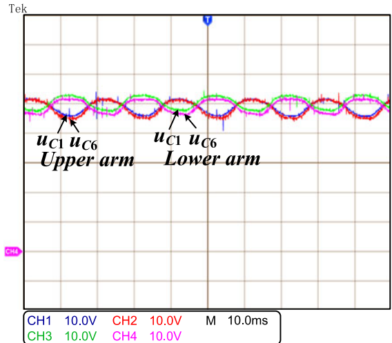
Fig. 25. Experimental capacitor voltage waveforms of SM 1 and SM 6 in each arm of phase A after compensation.
